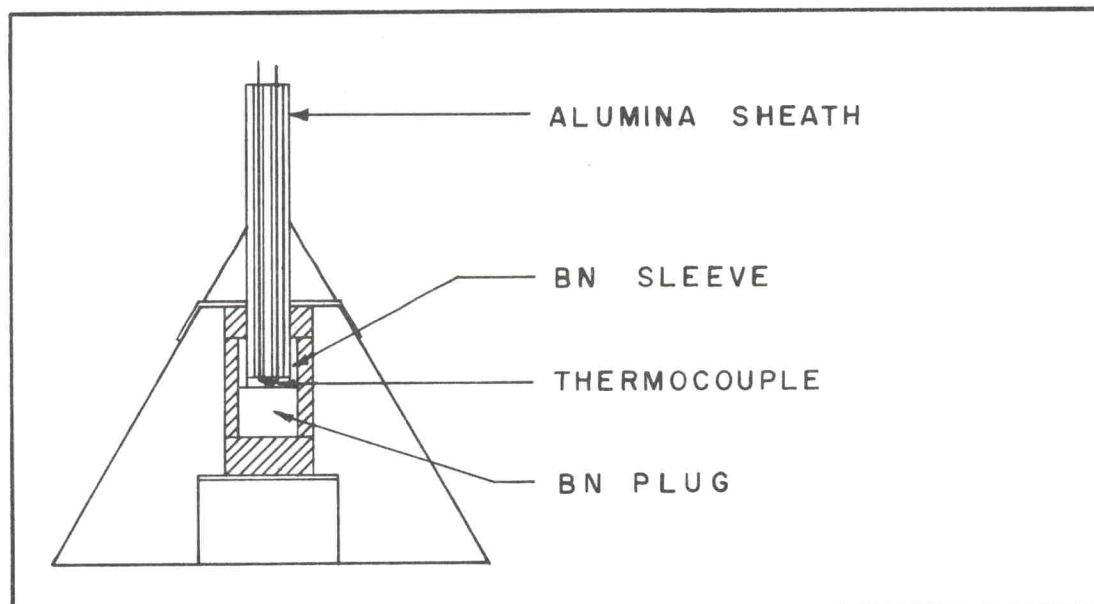
Figure 28. -Temperature Calibration Assembly No. 2.
